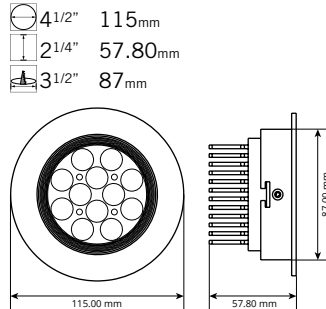
PL107-7W12LED
