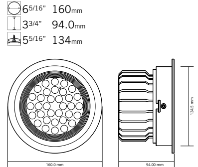
PL107-24W36LED
