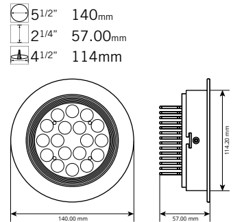
PL107-12W18LED
